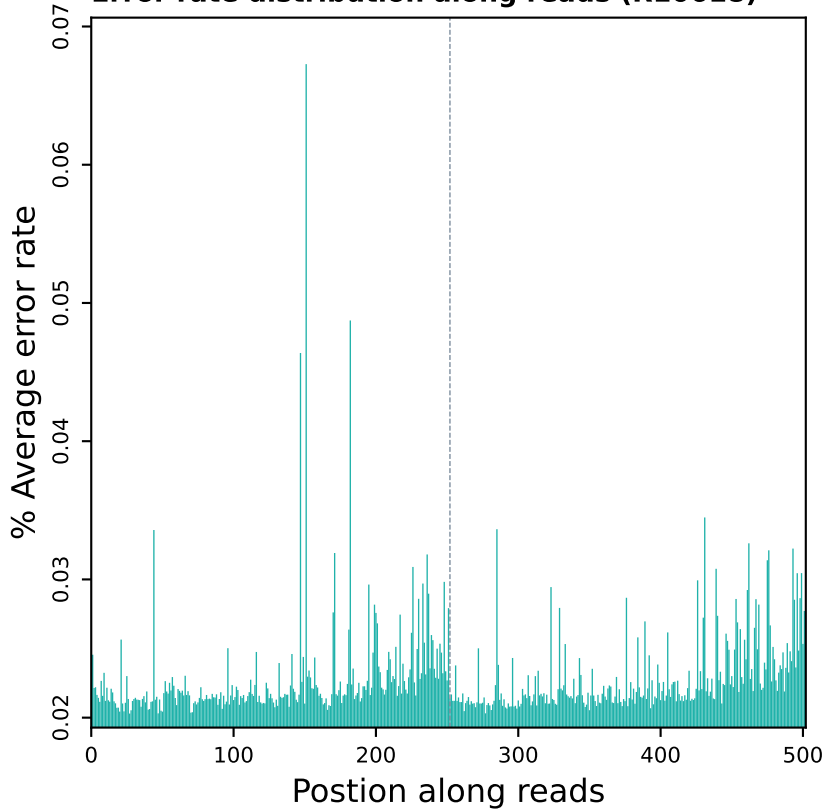
Error rate distribution along reads (R10618)
